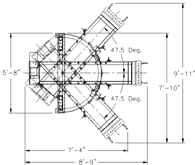
CTS730 Countertop Saw
